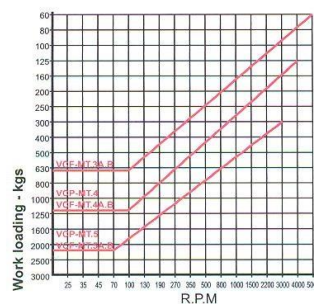
THE CHART FOR LOADING WEIGHT WITH R.P.M.
