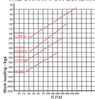
THE CHART FOR LOADING WEIGHT WITH R.P.M.
