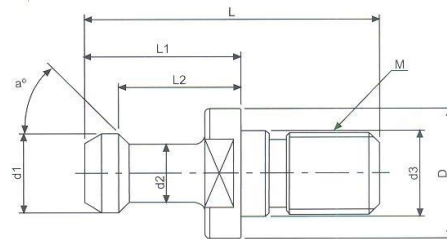
THREAD GROUND
