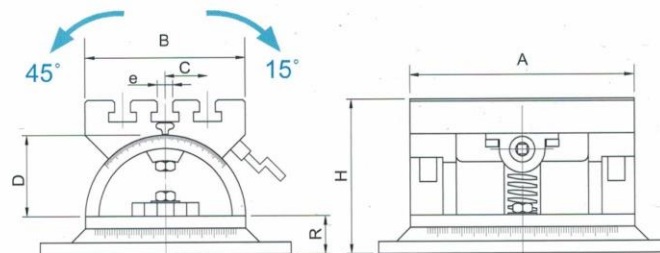
360° SWIVEL BASE.
