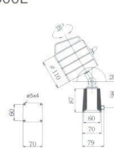
VHL-500S
