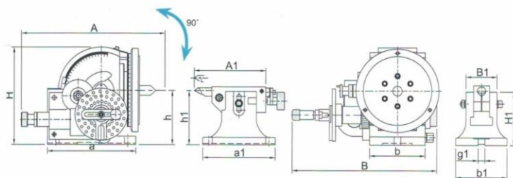
BS-2-J-8 THE CHUCK FIXING HOLE IS FROM FRONT.
